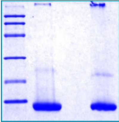
14% SDS-PAGE separation of Mouse Resistin 1. M.W. marker - 14, 21, 31, 45, 66, 97 kDa 2. reduced and heated sample, 2.5µg/lane 3. non-reduced and non-heated sample, 2.5µg/lane
